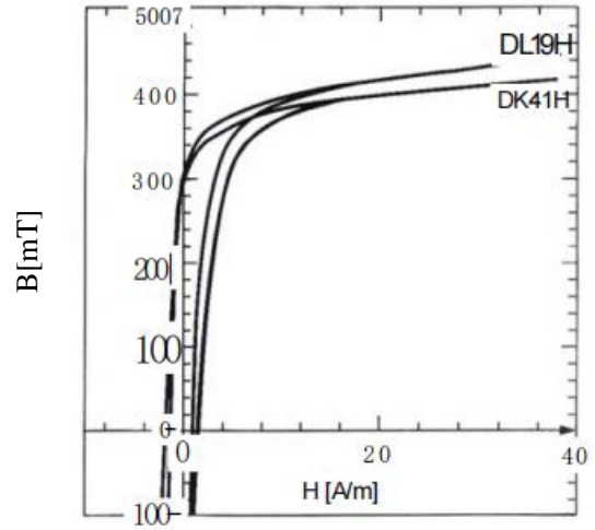
DK41H, DL19H B~H曲线
