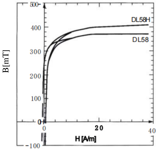
DL58, DL58H B~H曲线
